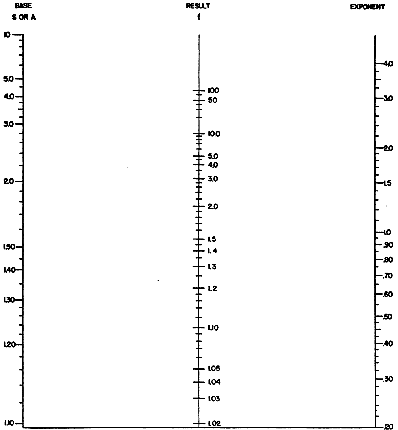
No. 2. NOMOGRAPH FOR RAISING BASE S OR A TO A FRACTIONAL EXPONENT
