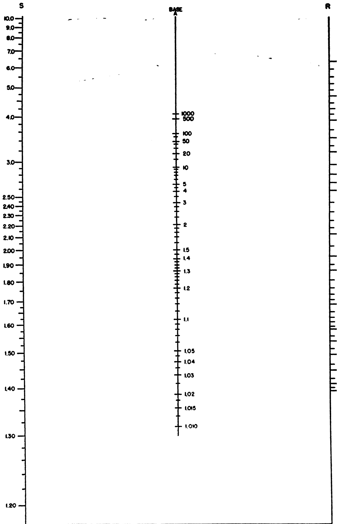
No. 3. NOMOGRAPH FOR OBTAINING BASE A
