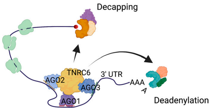
Fig. 1. Mechanisms of post-transcriptional gene repression mediated by the RISC. miRNAs guide the RISC to partially complementary binding sites within the 3' UTR of a target mRNA. Next, decapping and deadenylase complexes are recruited on the target mRNA. Upon deadenylation and decapping, mRNAs become substrate for cellular exonucleases and are rapidly degraded.
