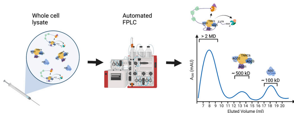
Fig. 2. SEC-based analysis of RISC size in whole cell and tissue lysates. Whole cell lysates are prepared as described in the main text, cleared by centrifugation, and loaded on a fast protein liquid chromatography automated system. One-milliliter fractions are collected, processed for trichloroacetic acid precipitation, and analyzed by Western blotting for detection of RISC components.
