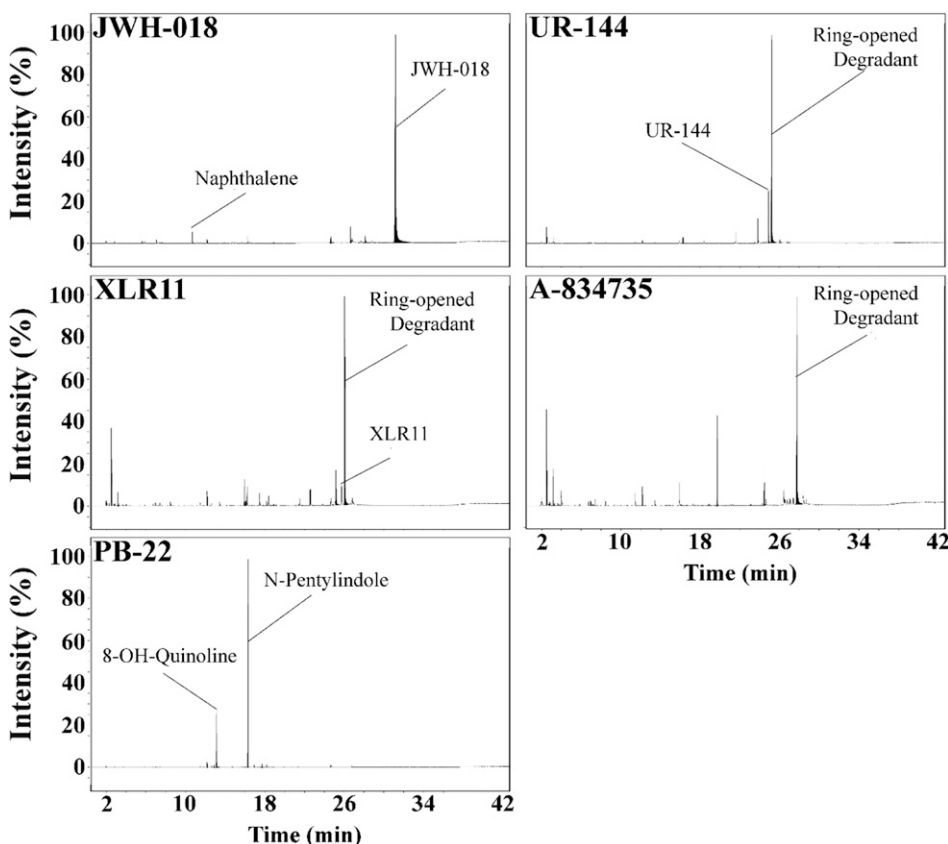
Fig. 1. Thermolysis of synthetic cannabinoids. Total ion chromatograms showing the results of aerobic thermolysis of JWH-018, UR-144, XLR-11, A-834735, and PB-22 at 800^{\circ}C . Note the differing degrees of degradation due to differences in chemical structure. Each chromatogram is shown plotted as normalized intensity (percentage) on the y-axis and elution time (minutes) on the x-axis.
