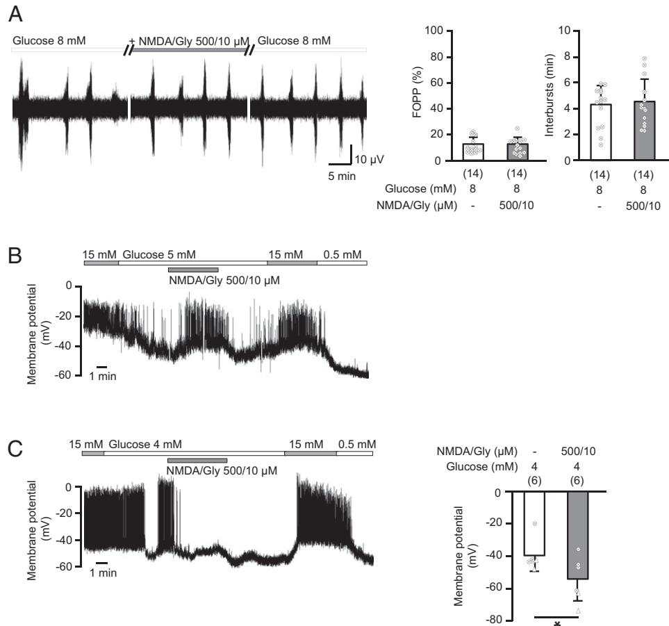
Fig. 3. Influence of NMDA on electrical activity of islets and \beta cells. (A) Acute application of NMDA/glycine (500 \mu M/Gly 10 \mu M) to whole islets cultured on microelectrode arrays did not change the fraction of electrical activity (FOPP) of islets stimulated by 8 mM glucose. An exemplary recording is shown on the left, the diagrams summarize the FOPP and the averaged interburst intervals of all experiments. (B and C) At a glucose concentration around the threshold for activation (4–5 mM), cells with a low frequency of action potentials (B) were depolarized by NMDA/glycine (500 \mu M/10 \mu M). By contrast, NMDA/glycine abrogated action potentials in those cells displaying higher frequency of action potentials (C). The diagram summarizes the changes in membrane potential in those cells that were hyperpolarized (six out of nine) by NMDA/glycine. The number of experiments with islets (A) of three different preparations (females) or islet cells of six preparations [B and C: female (circles)/male (triangles): four/two] is indicated in the diagrams. * P \leq 0.05 .
