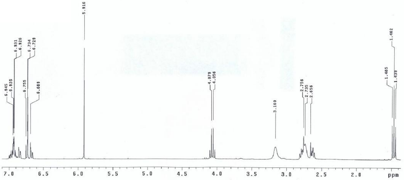
Supplemental Figure 2C. 1 H-NMR mass spectrum of LDT8.
