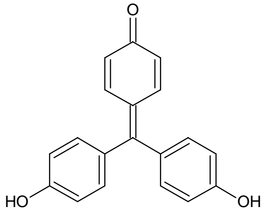
ROSOLIC ACID
