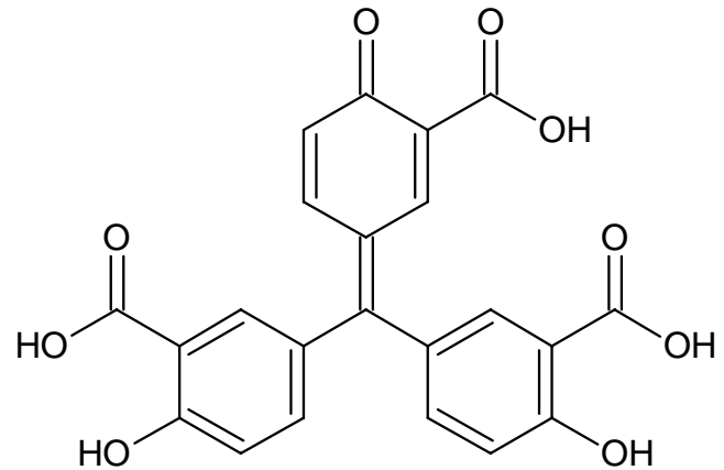
AURINTRICARBOXYLIC ACID
