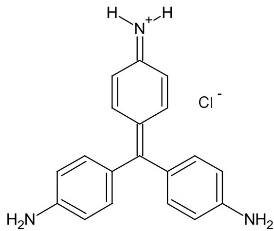
PARA-ROSANILINE CHLORIDE
