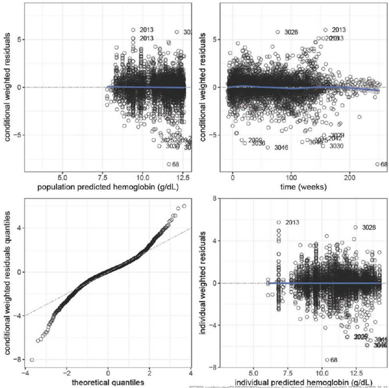
Supp. Fig. 7: The dashed line represents the identity line or zero line; the thick blue curve is the smoothing spline. Numbers indicate subject numbers with weighted residuals greater than 5 or less than -5.
