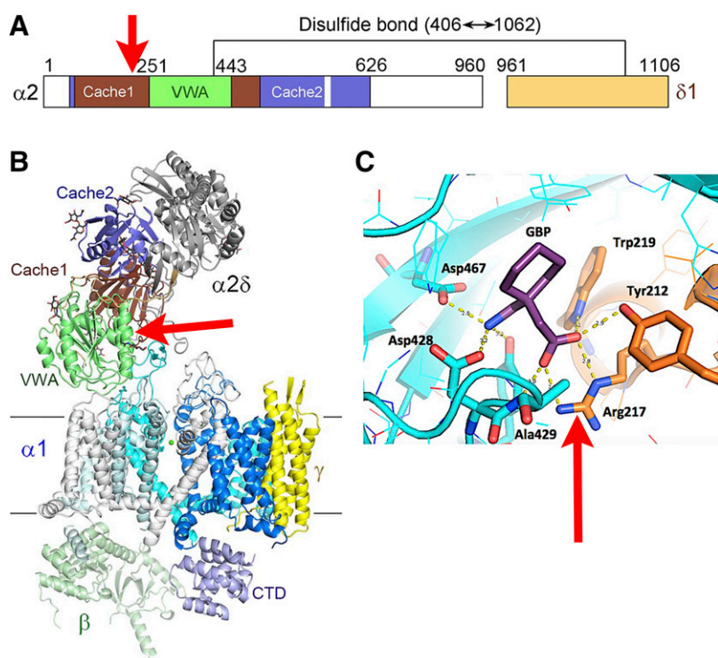
Fig. 1. Structures of the \alpha_2\delta -1 protein based on cryo-electron microscopy and molecular modeling (Wu et al., 2016) of calcium channels purified from skeletal muscle. (A) The numbered \alpha_2\delta -1 sequence with major domains colored [as in (B)]. The immature \alpha_2\delta -1 protein is cleaved (between residue 960 and 961), and the two resulting segments are joined by a disulfide bridge. The arginine at position 217 (Arg217) is critical for drug binding (see text) and is shown with a red arrow in each subpart of the figure. (B) Atomic resolution map of the entire voltage-gated calcium channel protein, including the ion-conducting \alpha_1 subunit (white and shades of blue for the four transmembrane domains), the \gamma subunit (yellow, which is not found in brain calcium channels), and the \beta subunit (pale green, on the cytosolic side of the membrane). The \alpha_2\delta -1 protein includes the VWA (green) with a MIDAS, Cache 1 and Cache 2 (brown and purple), and the C-terminal domain (CTD, purplish-gray). Some of the polysaccharide (glycan) groups are shown as abbreviated stick-figure sugar molecules. The R217 residue (red arrow) is buried in the middle of the protein between the VWA domain and the Cache 1 domain. (C) The presumed drug binding pocket (Kotev et al., 2018) consists in part of the Arg217 residue (red arrow), which coordinates with the acid moiety of gabapentin (GBP, purple). Other residues (numbered) coordinate with both the acid and the amine of gabapentin. It is presumed that drug binding to this pocket causes a large conformational change to \alpha_2\delta -1 that alters its interaction with other proteins. Figures are adapted from Wu et al. (2016) [parts (A) and (B)] with permission from AAAS and from Kotev et al. (2018) [part (C)], with permission from Journal of Chemical Information and Modeling, copyright (2016) American Chemical Society.
